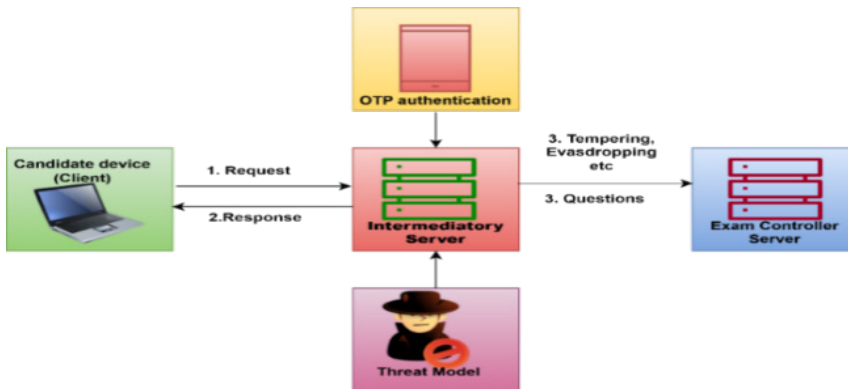
Figure 1 The Architectural Overview of the proposed model
