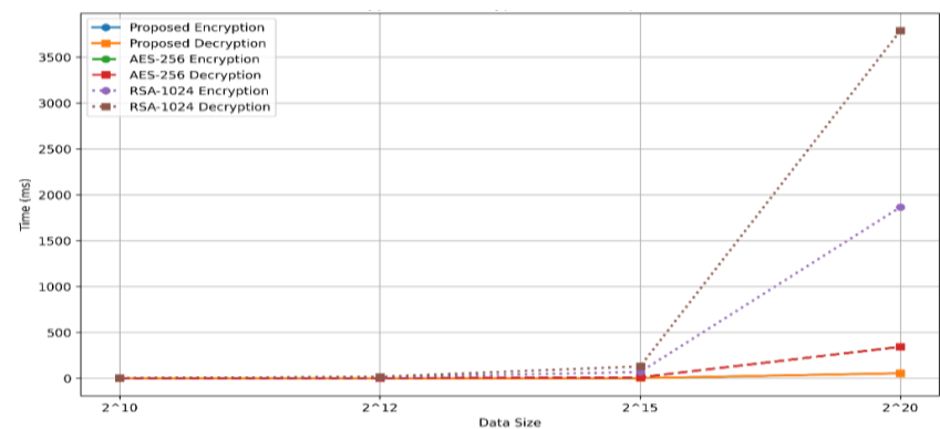
Figure 2 Encryption/Decryption Time (sec)
