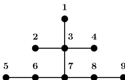
Figure 7 Prime Tree T_2 with 9 vertices.
