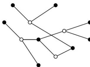
Figure 4 Arbitrary Tree T2 with 12 vertices
