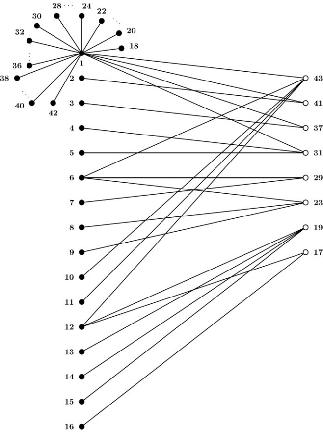
Figure 2 Construction of prime tree T' obtained after applying the prime labeling algorithm.
