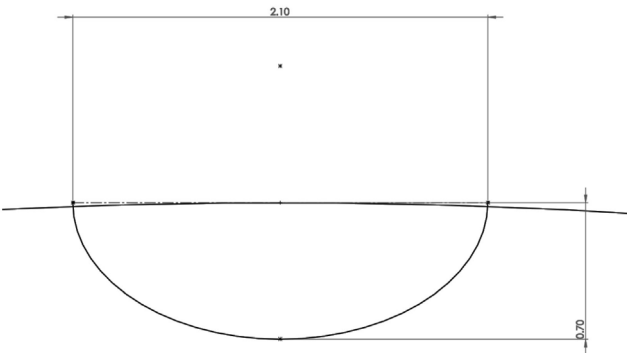
Figure 19 Elliptical Dimple Diagram
