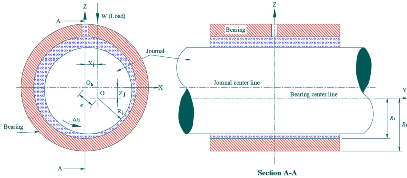
Figure 1 Schematic of a Hydrodynamic Journal Bearing
