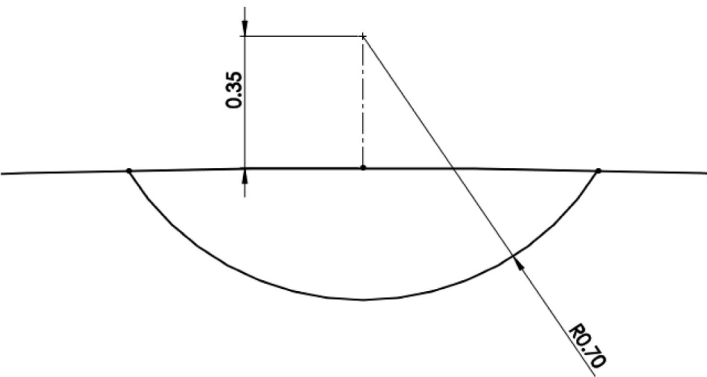
Figure 18 Shallow Dimple Diagram
