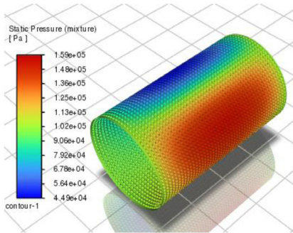
Figure 25 Elliptical Dimple Textured Bearing Pressure Contour
