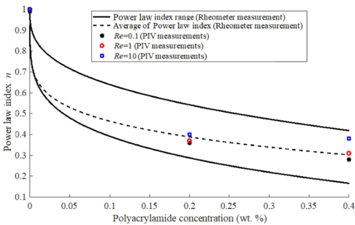
Figure 3 Polyacrylamide concentration vs power law index [25]
