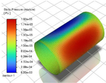
Figure 24 Shallow Dimple Textured Bearing Pressure Contour
