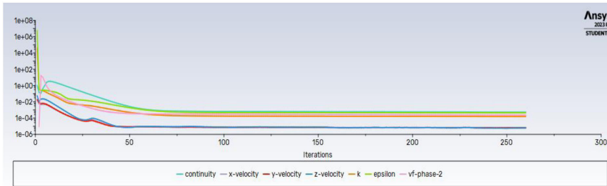
Figure 6 Residual convergence
