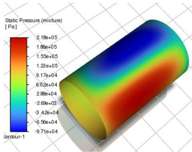
Figure 9 Pressure Contour achieved during CFD Analysis
