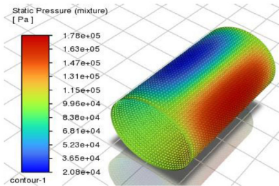
Figure 23 Hemispherical Dimple Textured Bearing Pressure Contour
