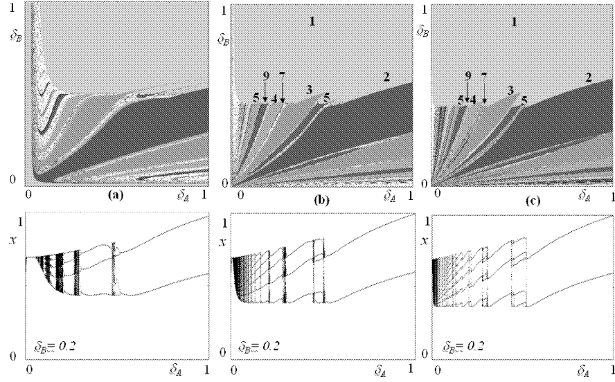
FIGURE 7. Bifurcation diagrams in the parameters' plane (\delta_A, \delta_B) for the continuous map g(z) = \frac{2}{\pi} \arctan(\lambda z) with (a) \lambda = 100 (b) \lambda = 600 (c) \lambda = 5000 . The grey shaded regions represent periodic tongues of low periods, whereas in the white regions the asymptotic behavior is periodic with high periods or aperiodic, i.e. chaotic, as shown in the corresponding one-dimensional bifurcation diagrams shown in the lower part of the figure, obtained with increasing values of \delta_A and a fixed value \delta_B = 0.2 .
