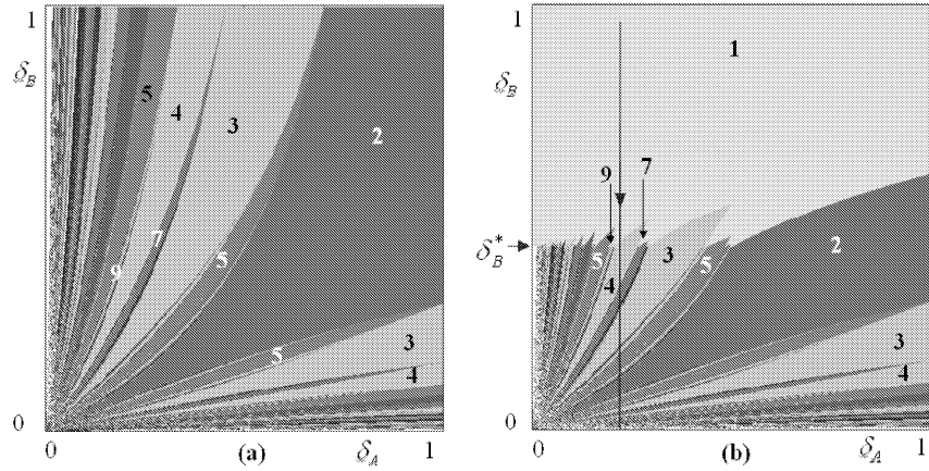
FIGURE 2. Two-dimensional bifurcation diagrams in the plane (\delta_A, \delta_B) of the map T . In (a) d_1 = 0.0 and d_2 = 0.7 . In (b) d_1 = 0.4 and d_2 = 0.7 .
