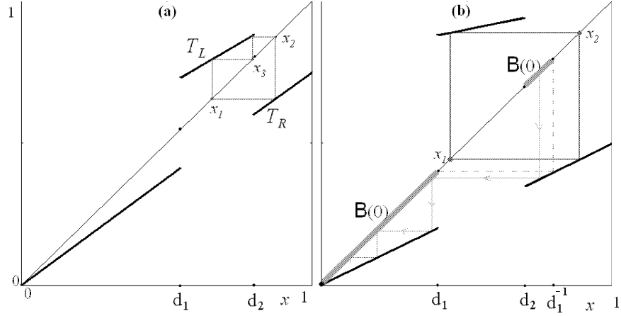
FIGURE 1. Map (4), coexistence of two attractors. (a) With parameters m_1 = 0.75 , m_2 = 0.6 , d_1 = 0.55 , d_2 = 0.8 , the two attractors are the origin and a cycle of period 3. (b) With parameters m_1 = 0.5 , m_2 = 0.2 , d_1 = 0.4 , d_2 = 0.7 the two attractors are the origin and a cycle of period 2.
