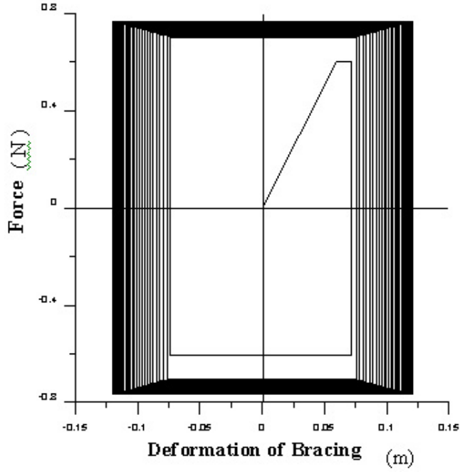
FIGURE 12. The hysteresis loop of bracing for structure w/ ASHD. (k_{str} = 100N/m, k_b = 10N/m, k_a = 0.7N/m, P_a = 0.6N)
