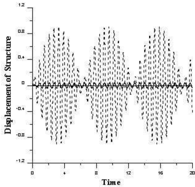
FIGURE 2. Time history of structural displacement for structure w/ and w/o ASHD
