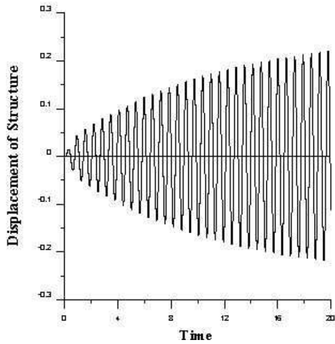
FIGURE 8. The time history of post stage of resonance behavior for structural displacement of structure w/ ASHD.
