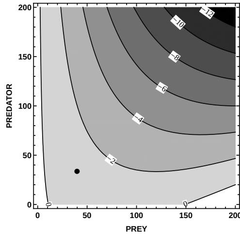
FIGURE 1. A contour plot of the deviation curvature of the predation system as a function of the number of population of the prey and that of the predator. The filled circle is the equilibrium point.
