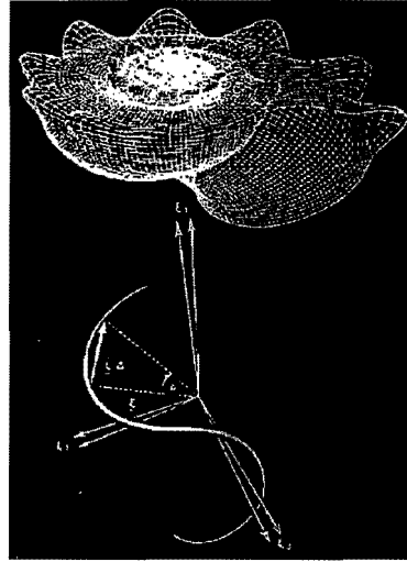
FIGURE 4. An illustration of the fourth scientific imbalance of the 20th century, the representation of biological structures (including cells, organisms and their functions) via a mathematics which is not only Hamiltonian and reversible, but also single valued, while said biological systems require a mathematics which is not only nonhamiltonian and irreversible, but also multi-valued, as illustrated by the growth of a sea shell which, besides not being representable with a Hamiltonian and being irreversible, requires the doubling of all Euclidean reference axes.
