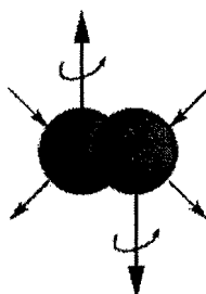
FIGURE 2. An illustration of the second scientific imbalance of the 20-th century, the lack of adequate mathematics for quantitative studies of nonlocal-integral interactions occurring in the deep overlappings of the wavepackets of electron valence bonds in molecules, as well as, in general, all interactions of particles at short distances.
