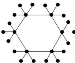
Figure 2 The thorn cycle C_6 \circ \bar{K}_3 .
