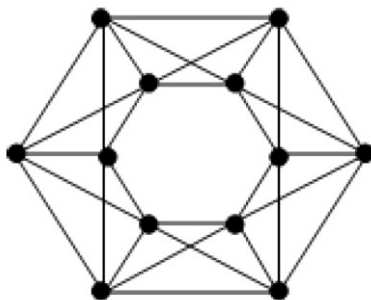
Figure 6 The closed fence graph C_6[K_2] .
