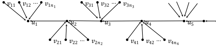
Figure 2 The non-homogeneous converging caterpillar graph
